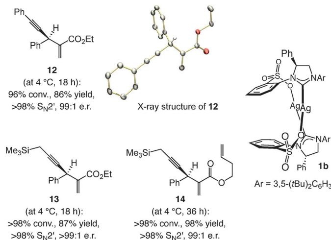
Scheme 3. Additional products of high enantiomeric purity obtained through EAS with alkynylaluminum reagents and the catalyst precursor used to generate them. Reactions were performed under conditions shown in Table 1.
