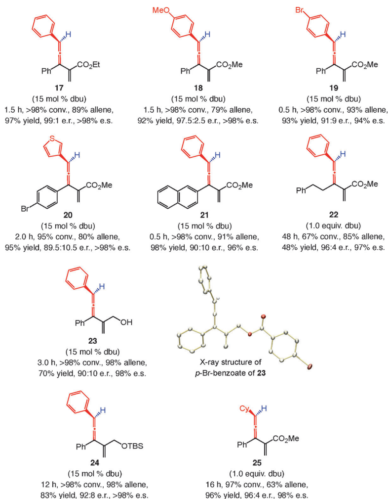
Scheme 5. Trisubstituted allenes can be accessed efficiently in high enantiomeric purity through dbu-catalyzed isomerization; the X-ray structure of a derivative of 23 supports the syn mode of proton transfer. Yields correspond to mixtures of isomers.
