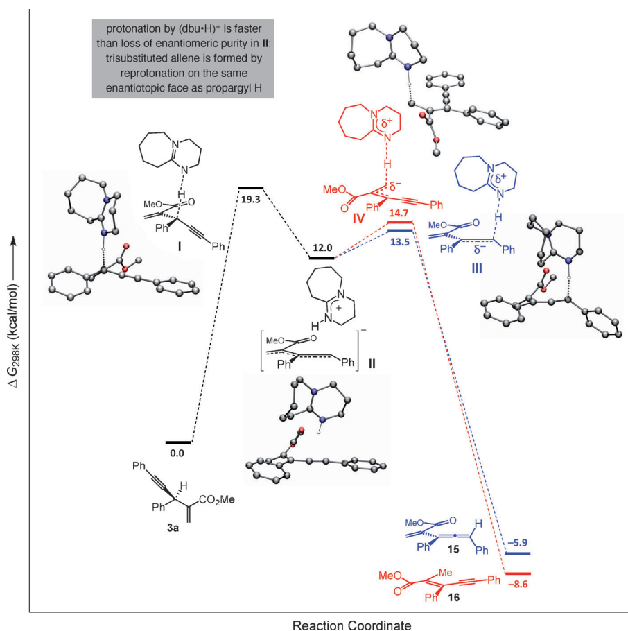
Scheme 6. DFT calculations indicate that, with dbu as base, the deprotonation step might be rate limiting and generation of the allene product is kinetically preferred although the tetrasubstituted alkene is thermodynamically favored. See the Supporting Information for details.
