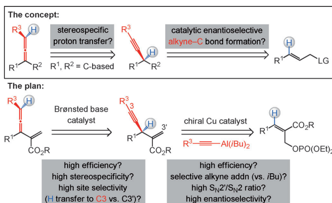
Scheme 1. Strategy for synthesis of enantiomerically enriched trisubstituted allenes by stereospecific transformation of an appropriate alkynyl substrate accessed through catalytic EAS with alkynylaluminum reagents as nucleophiles. LG = Leaving group.
