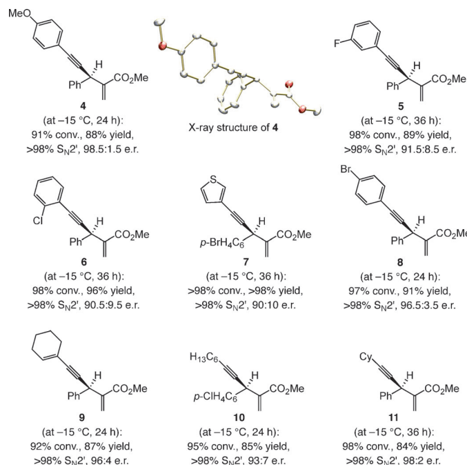
Scheme 2. A range of products can be accessed in high efficiency and site- and enantioselectivity through catalytic EAS. Reactions were performed under the conditions shown in Table 1 ( 1a as catalyst precursor); 0.5 mol % 1a and 1.0 mol % Cu salt used for EAS affording 7 and 11 .
