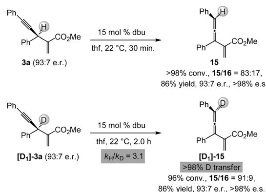
Scheme 4. Alkyne-to-allene isomerization proceeds to completion within 30 min; labeling experiment indicates a significant primary kinetic isotope effect. Yields correspond to mixtures of isomers; see the Supporting Information for details.
